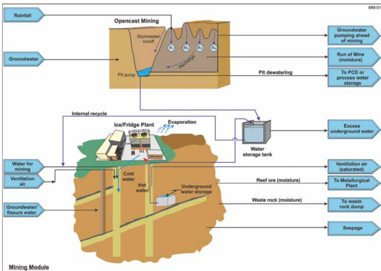
Figure C2: Mining section water balance diagram
