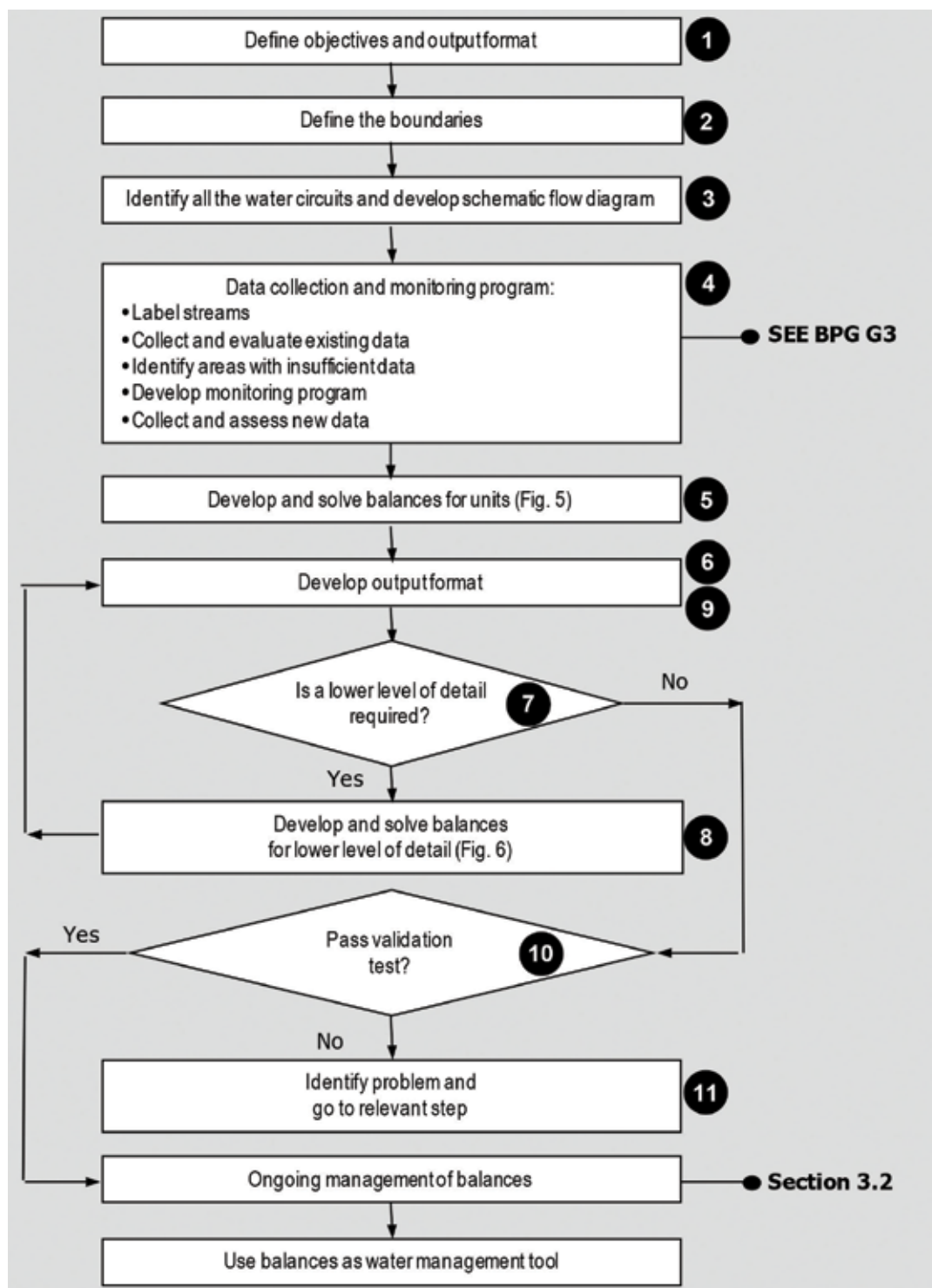
Figure 3: Methodology for development of a water balance (source BPG G2)
