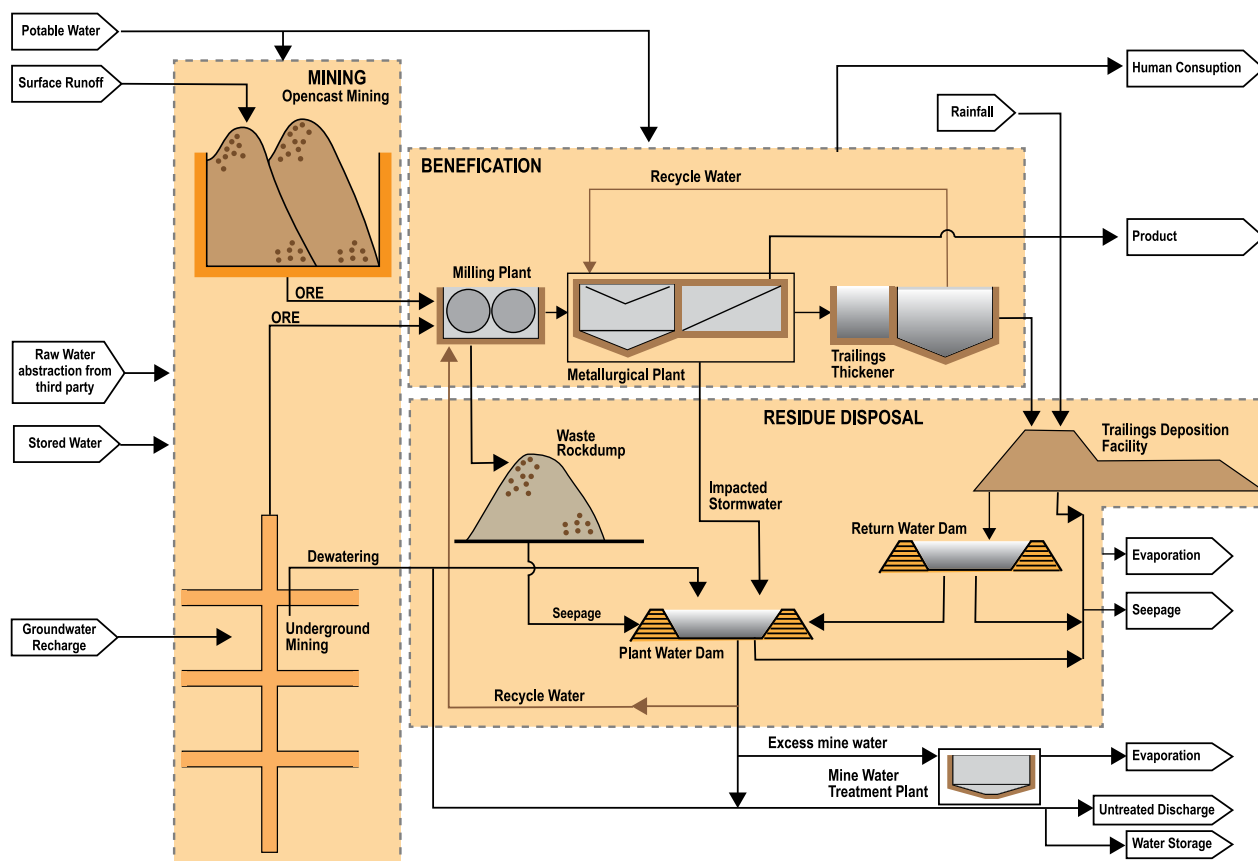
Figure 10: Case study water balance flow diagram/ schematic
